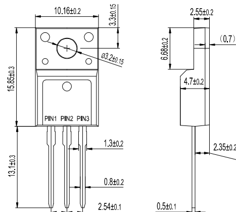
ITO-220AB FR16XXFCT
