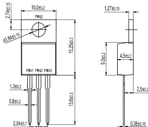
TO-220AB FR16XXCT
